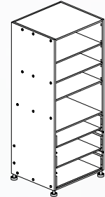
3 DRAWER PANTRY CABINET 600mm, internal drawers
